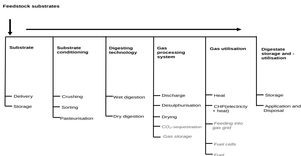
Figure 7.1 Process steps of biogas technologies (LfU 2007)
