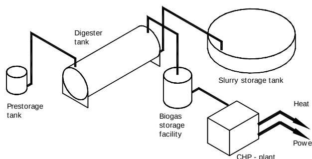
Figure 4.2 Schematic representation of a farm scale biogas plant, with horizontal digester of steel. (HJORT-GREGERSEN 1998)
