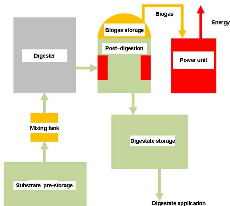
Figure 7.2 Main components and general process flow of biogas production (PRA&L 2008)
