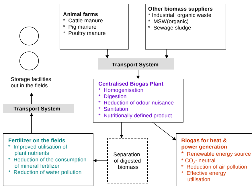
Figure 4.10 The integrated concept of centralised co-digestion plant
